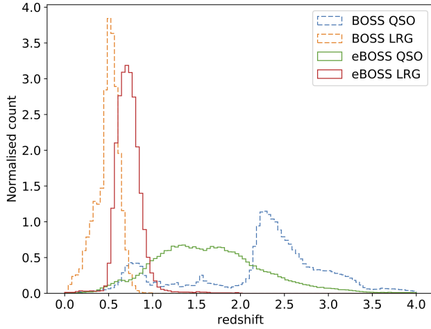
FIG. 1.— N(z) of eBOSS DR14 QSO and LRG compared to DR12 BOSS, demonstrating how eBOSS is filling in the redshift desert between z \sim 0.8 - 2.0 .
